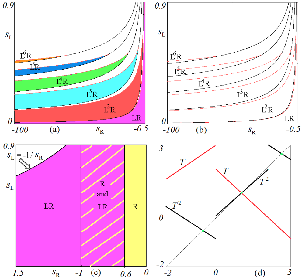
Figure 2: Two dimensional (s_R, s_L) bifurcation diagram in (a) and related BCB curves in (b), at m_L = 3 and m_R = 2 . The enlarged portion for -1.5 < s_R < 0 is shown in (c) where the coexistence region occurs for -1 < s_R < -m_R/m_L = 0.\bar{6} . In (d) the shape of the map and of its second iterate are presented.
