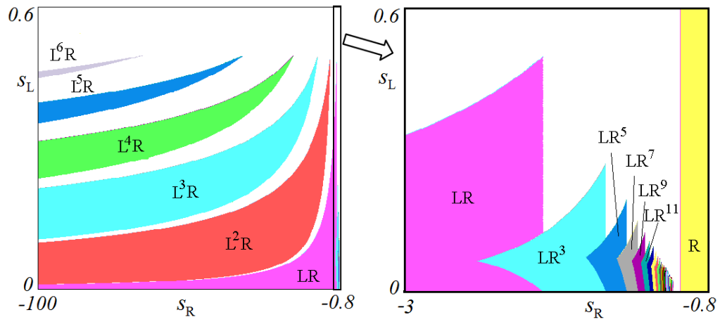
Figure 3: Two-dimensional orbit diagram at m_L = 1 and m_R = 2 .
