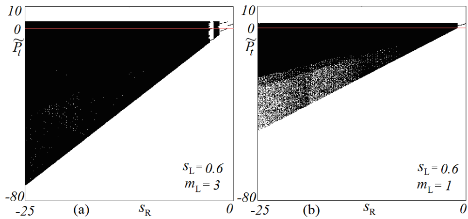
Figure 4: Bifurcation diagrams.
