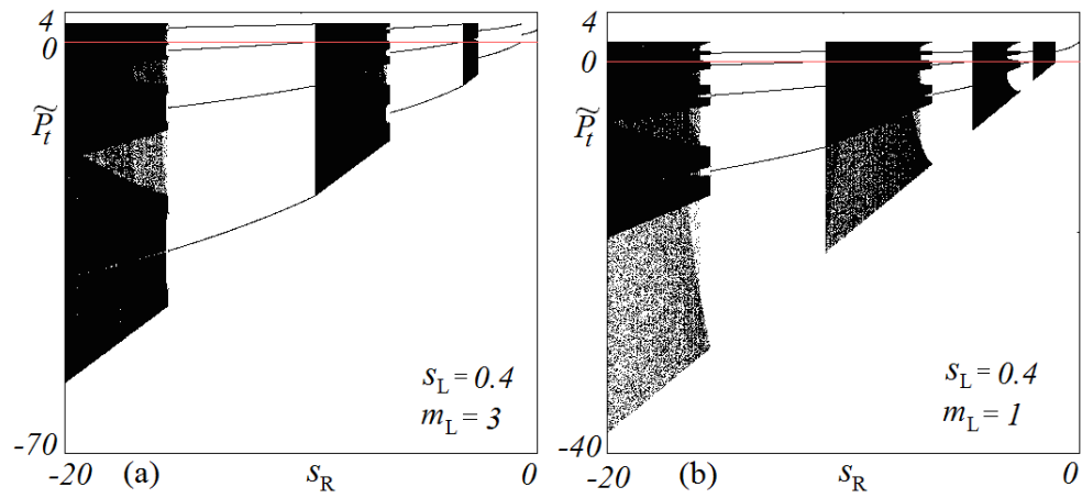
Figure 5: Bifurcation diagrams.
