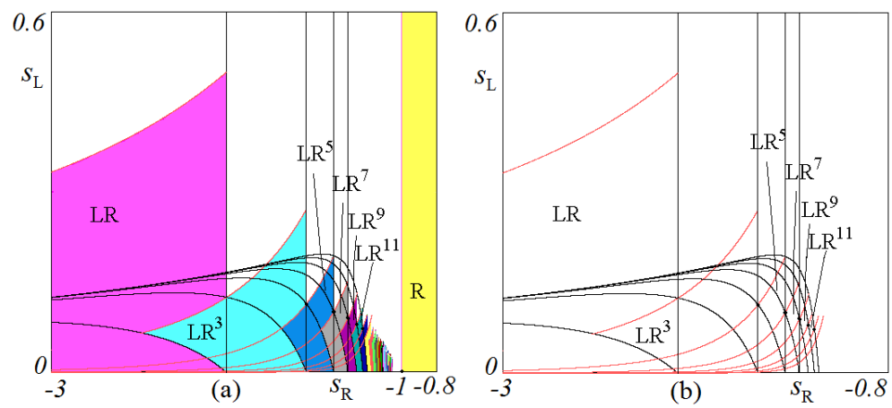
Figure 8: Two-dimensional orbit diagram.
